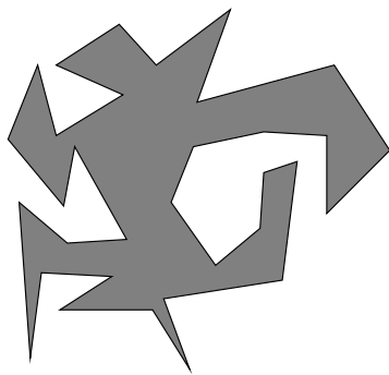
OK
