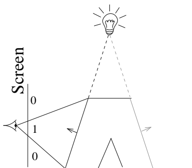
Front facing +1
