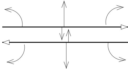
Half-edge
