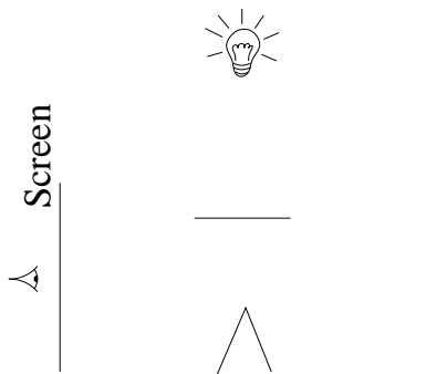
Scene
