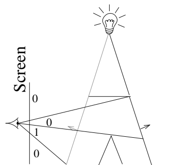
Back facing -1
