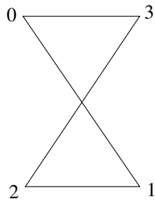
Line crossing
