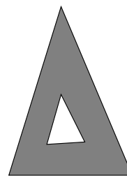
Hole
