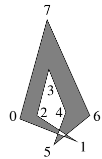
Overlapping
