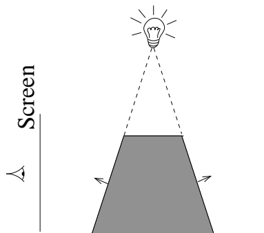
Shadow Volume
